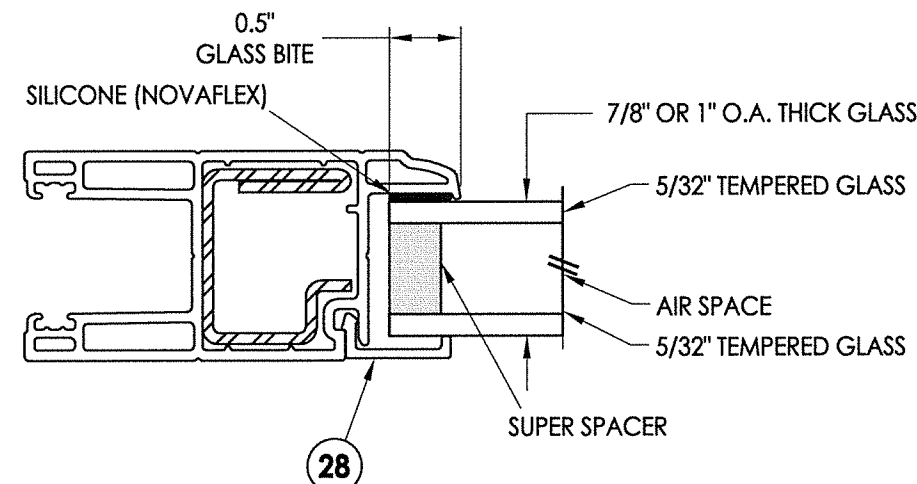
G2 GLAZING DETAIL INTEGRAL 7/8" OR 1" IG
