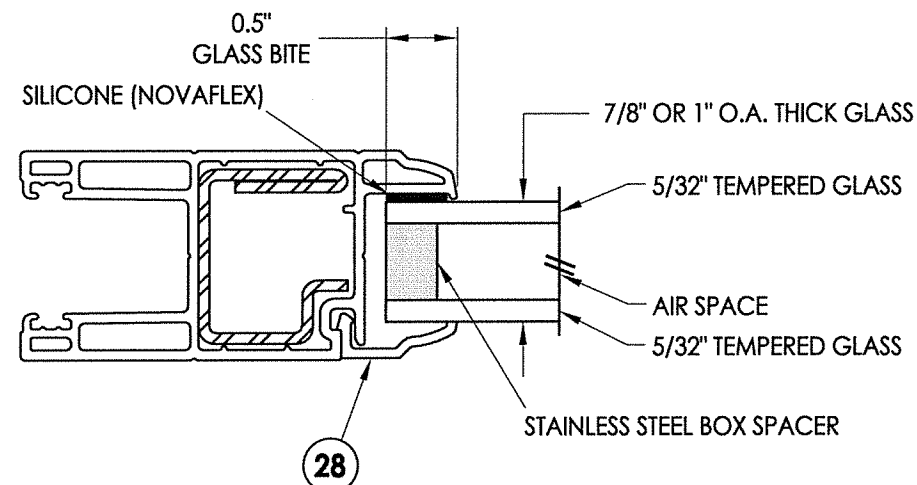
G1 GLAZING DETAIL CARDINAL 7/8" OR 1" IG
